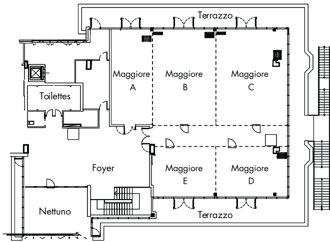
PRIMO PIANO FIRST FLOOR
